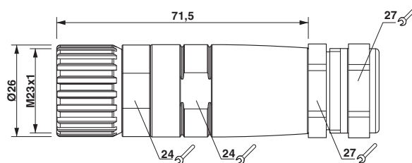
Dimensional drawing
